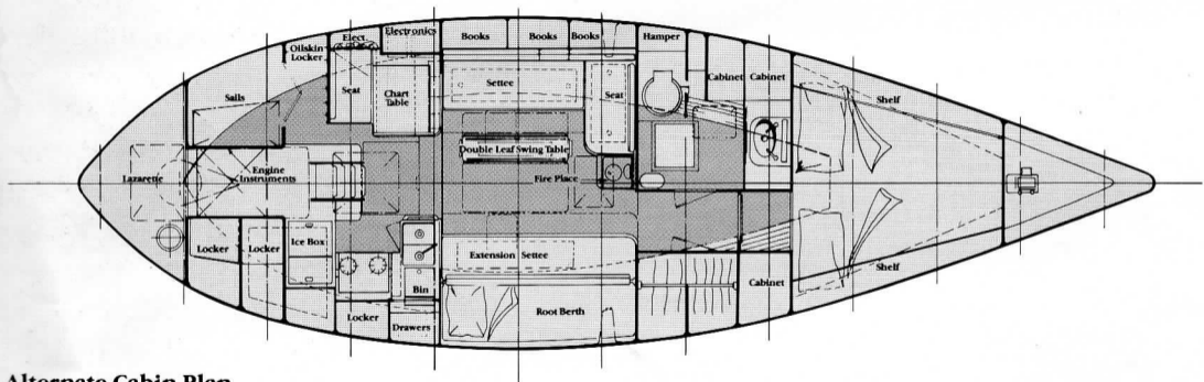
Alternate Cabin Plan
